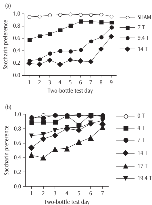
Figure 20.3. Magnitude and persistence of CTA is proportional to magnetic field strength, as shown by extinction during consecutive 24-h, two-bottle preference tests. (a) Extinction curves after three pairings of 10-min access of G + S with 30-min exposure within 7 T, 9.4 T, or 14 T superconducting magnets. Repeated pairings with 7 T were sufficient to significantly decrease G + S preference. (b) Extinction curves after one pairing of 10-min access of G + S with 30-min exposure within a 0–19.4-T magnetic field of a resistive magnet. Maximal CTA was observed after 17-T exposure.
