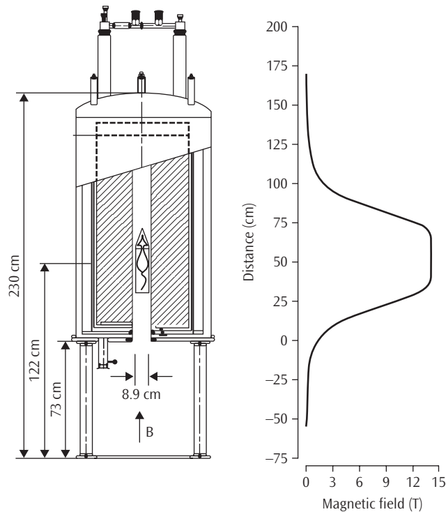
Figure 20.1. Cross-sectional schematic of the 14.1-T superconducting magnet (a) and the corresponding magnetic field (b) relative to the opening of the magnet's bore at 0 cm. Rats were restrained in Plexiglas cylinders and inserted vertically within the bore. Note that while the maximum field is found at the center of the magnet, there are large magnet field gradients (T/m) where the magnetic field strength is rapidly changing. Maximum effects on CTA and other measures were induced, however, when the rats were within the uniform 14.1-T field that extends approximately 15 cm around the center of the magnet's bore.
